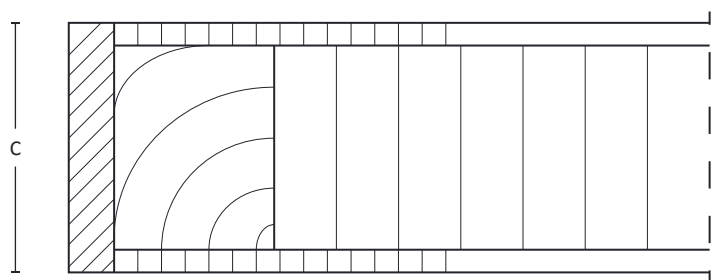
HORIZONTAL CUT
